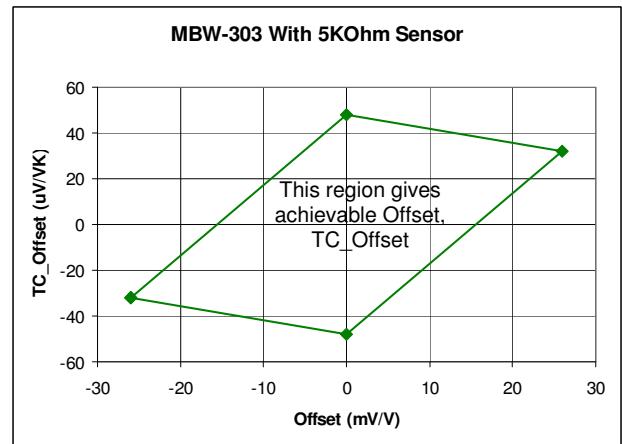
Figure 3: MBW-303 With 5kΩ, +2400ppm/K Sensor
