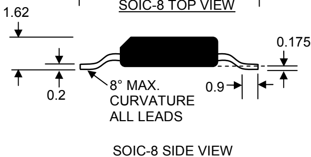
Figure 9: Package Dimensions
