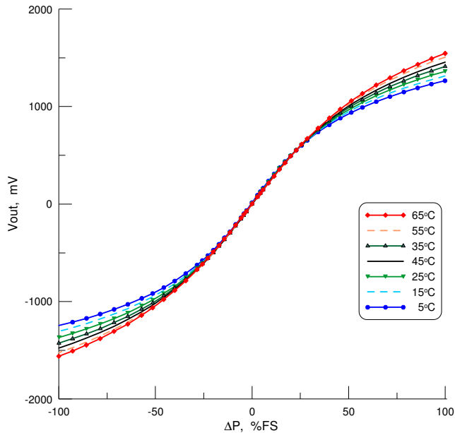
Fig. 5: Typical deviation of V_{out} vs. \Delta P with temperature for MB-LPS2-03 sensors. While all curves, from 5°C to 65°C coincide at Low- \Delta P , up to \pm 20\% of Full-Scale pressure span, the curves then diverge to a wider tolerance at \pm Full-Scale pressure span.
